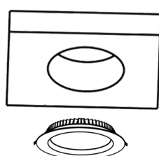
Europa 1 article: 241504/241514 Cut-out: Ø170-180mm
