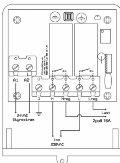
2-polt kobling
