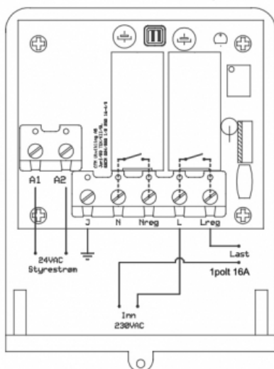
1-polt kobling
